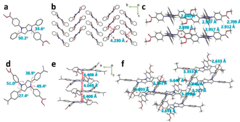
Fig. 6 The crystal structure, packing patterns, and intermolecular interactions of DPP-1MF (a, b, and c) and DPP-1MF-2IP (d, e, and f), respectively. (Hydrogen omitted for clarity (a, b, d, and e).)
