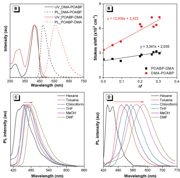
Fig. 1 (A) Normalized UV-vis absorption and PL spectra of the organoboron compounds in THF (10 μM). (B) Lippert–Mataga plots of Stokes shifts versus the solvent orientation polarizability of DMA-POABP and POABP-DMA. (C and D) Normalized PL spectra of (C) DMA-POABP and (D) POABP-DMA in different solvents.
