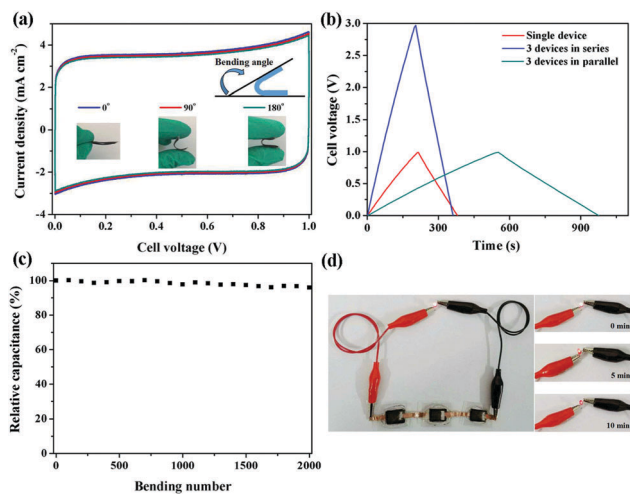
Fig. 6 (a) CV curves of the flexible supercapacitor at different bending angles at the scan rate of 20 mV s -1 ; (b) GCD curves of a single device and three devices connected in series and parallel at 0.3 A cm -2 ; (c) the relative capacitance of the flexible supercapacitor after different bending cycles; (d) photographs of three connected devices in series powering a red LED.
