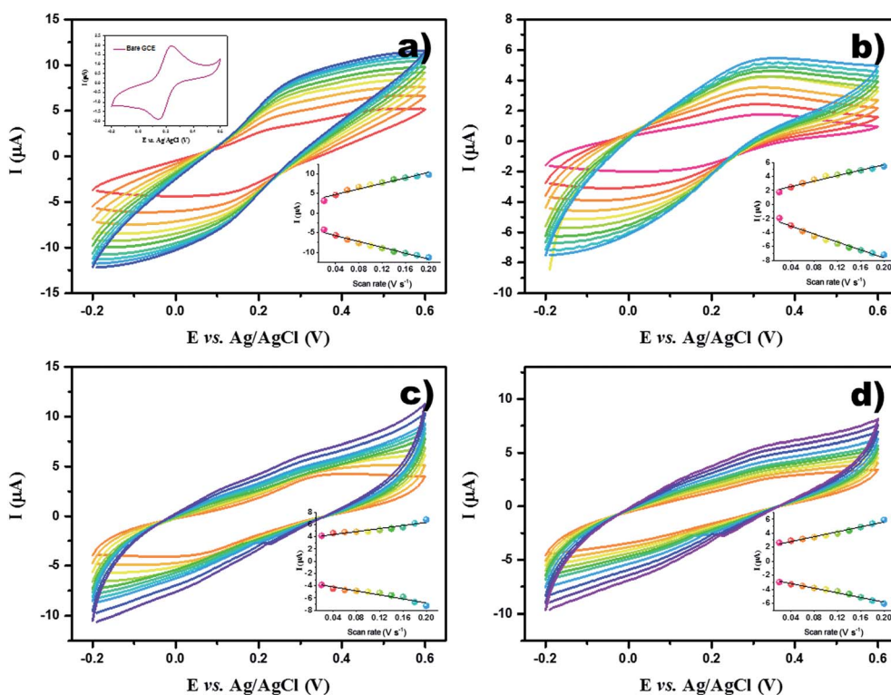
Fig. 4 CV curves for 5\text{ mM} of \text{Fe}(\text{CN})_6^{3-/4-} ( 0.1\text{ M KCl} ) at different scan rate from 0.02\text{ V s}^{-1} to 0.20\text{ V s}^{-1} at the modified electrodes GCE/TiO 2 NW/PAPBA–Au TNC (a), GCE/PAPBA–Au NC (b), GCE/TiO 2 NW/PAPBA NC (c), GCE/pristine PAPBA (d) and bare GCE (a, inset).
