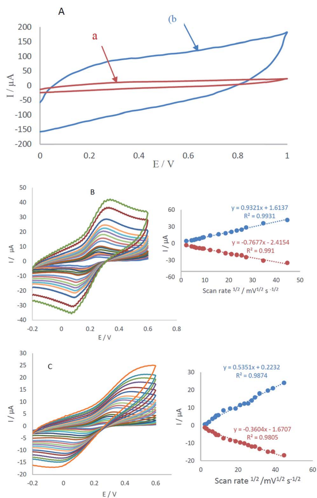
Fig. 2 (A) Electrochemical behavior of (a) CCME and (b) MCCME-BB in PBS (pH 4.0) at a scan rate of 50 \text{ mV s}^{-1} and CVs of (B) MCCME-BB and (C) CCME of 10 \text{ mM } [\text{Fe}(\text{CN})_6]^{3-/4-} prepared in 0.1 \text{ M KCl} at different scan rates, insets; plots of I vs. \nu^{1/2} of B and C, respectively).
