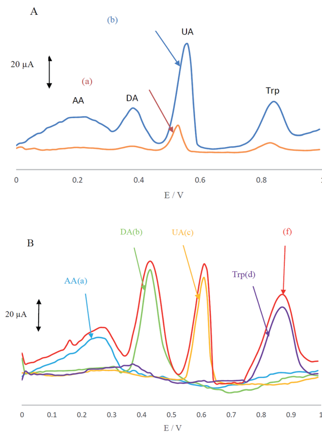
Fig. 3 (A) Differential pulse voltammograms of (a) CCME and (b) MCCME-BB in PBS (pH 4.0) containing AA ( 400 \mu\text{M} ), DA ( 200 \mu\text{M} ), UA ( 200 \mu\text{M} ) and Trp ( 200 \mu\text{M} ) and (B) differential pulse voltammograms of MCCME-BB for individual solutions of (a) AA, (b) DA, (c) UA, (d) Trp and (f) a mixture of AA, DA, UA, Trp.
