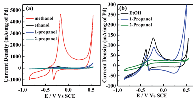
Fig. 4 (a) CV curves from: the Pd-Cu/C electrocatalyst for C 1 –C 3 aliphatic alcohol (1 M) oxidation in KOH (1 M) solution; and (b) Pd-Cu/C in 1 M EtOH, 1-propanol and 2-propanol at a scan rate of 50 mV s -1 at room temperature.
