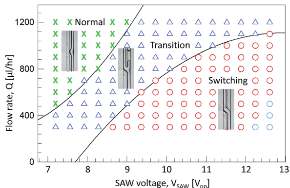
Fig. 5 A regime diagram of the acoustic flow switching by controlling the flow rate and the SAW voltage. The symbols 'x', 'Δ', and 'o' represent the normal, transition, switching regime, respectively. The blue symbol 'o' indicates the unstable flow switching regime. The transition lines between the each regime were roughly estimated.
