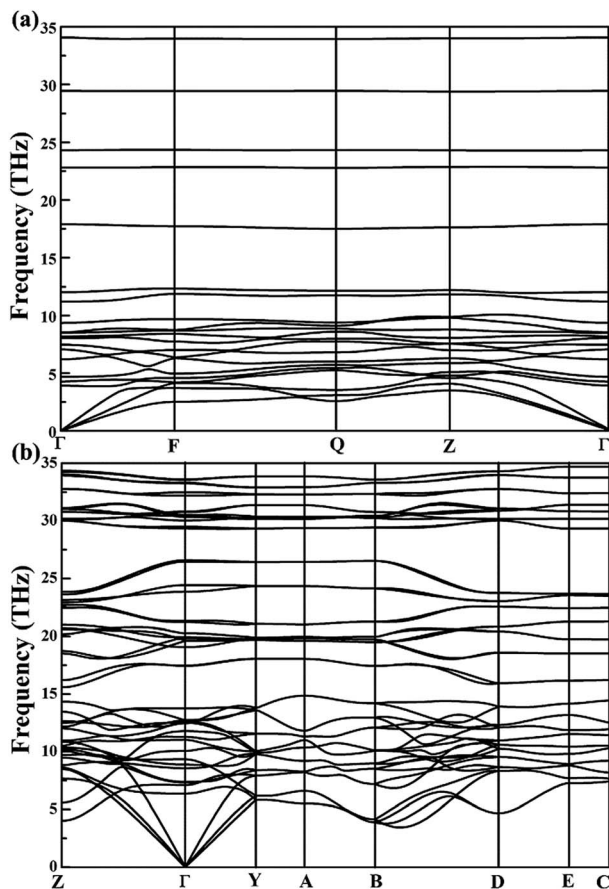
Fig. 2 Phonon dispersion curves for (a) P\bar{1} - \text{CaN}_3 at ambient pressure and (b) C2/m - \text{CaN}_3 at 60 GPa.
