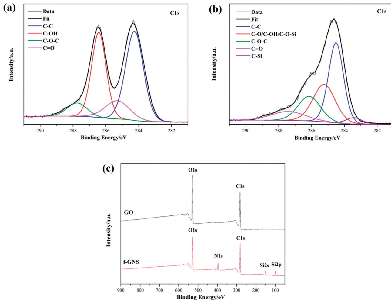
Fig. 3 \text{C}_{1\text{s}} XPS spectra of (a) GO, (b) f-GNs and (c) wide region XPS spectra.
