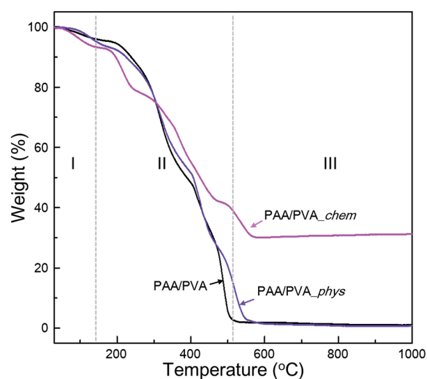
Fig. 3 Thermogravimetric curves of pristine nanofibrous film and the physically and chemically assembled nanofibrous film with functionalized BNNTs under aerobic condition.
