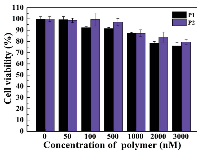
Fig. 4 CCK-8 viability assay of HeLa cells treated with two different gene vectors under different concentrations.
