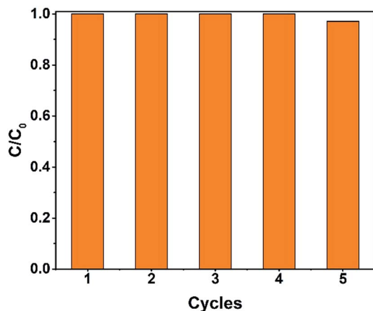
Fig. 12 The recycling test of the \text{Fe}_2\text{O}_3@DTT to degrade orange II (15 mg catalyst, 30 ml orange II, 12 mM \text{H}_2\text{O}_2 , 6 mM \text{NH}_2\text{OH}-\text{HCl} , irradiation times 1 h and at room temperature).
