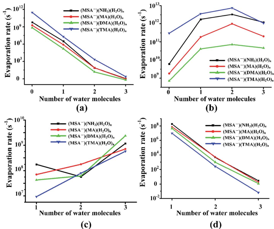
Fig. 5 Evaporation rates from the (MSA - )(NH 3 /amines)(H 2 O) n ( n = 0-3 ) clusters. The top left (a), top right (b), bottom left (c) and bottom right (d) panels give the results for evaporation of MSA - , NH 3 /MA/DMA/TMA, H 2 O and (MSA - )(NH 3 )/(MSA - )(MA)/(MSA - )(DMA)/(MSA - )(TMA), respectively.
