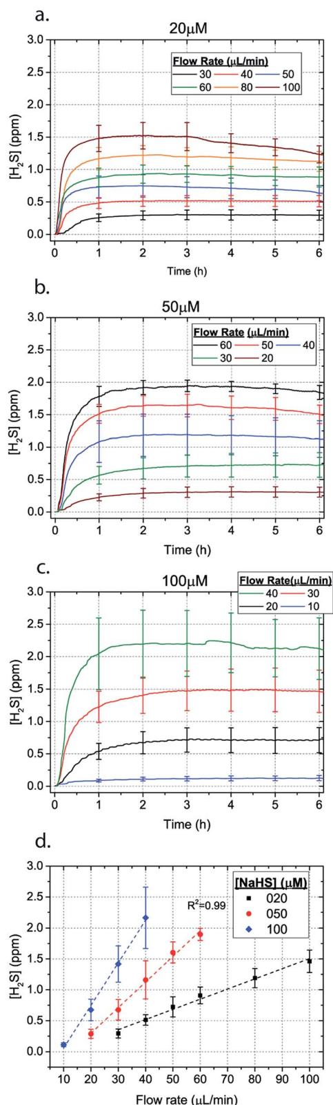
Fig. 3 H_2S concentration for different flow rates for (a) 20 \mu M (b) 50 \mu M and (c) 100 \mu M NaSH (error bars shown every hour). The average between 1–6 hours for different flow rates is depicted in (d).
