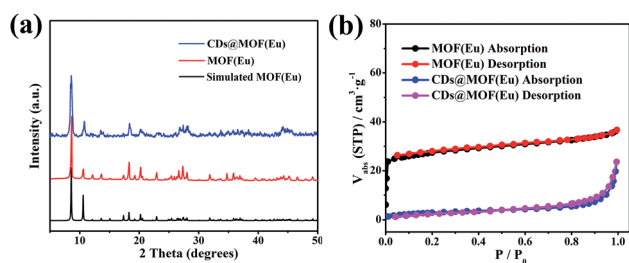
Fig. 2 (a) Comparison of the XRD patterns of MOF(Eu) and CDs@MOF(Eu) composite. (b) \text{N}_2 absorption–desorption isotherms of MOF(Eu) and CDs@MOF(Eu).
