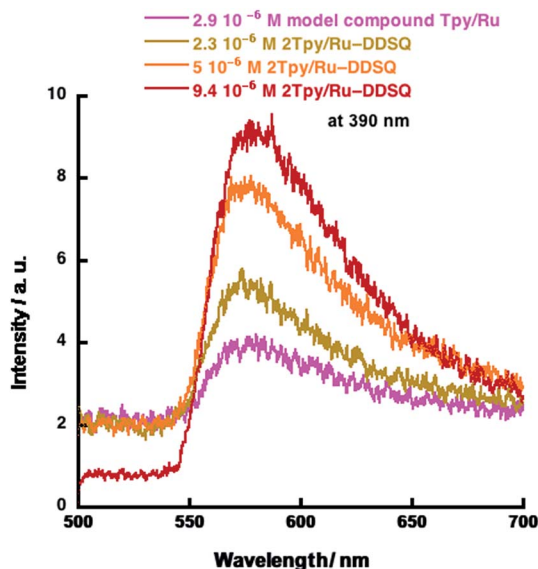
Fig. 6 Emission spectra of the model compound Tpy/Ru and 2Tpy/Ru- DDSQ with different concentrations. Three different wavelengths of 390 nm, 400 nm and 410 nm are used as the excitation wavelengths for 2Tpy/Ru- DDSQ.
