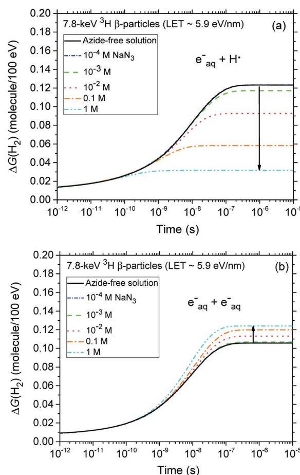
Fig. 4 Time dependence of the extents \Delta G(H_2) (in molecule/100 eV) of the reactions ( e_{aq}^- + H^{\bullet} ) (panel a) and ( e_{aq}^- + e_{aq}^- ) (panel b) that contribute to the formation of molecular hydrogen, calculated from our Monte Carlo simulations of the radiolysis of air-saturated aqueous azide ( NaN_3 ) solutions (pH neutral, 25 ^{\circ}C ) by 7.8 keV ^3H \beta -particles (LET \sim 5.9 eV nm ^{-1} ) in the time interval 1 ps to 10 \mu s. The blue, green, red, orange, and cyan lines correspond to the five different concentrations of azide anions studied: 10^{-4} , 10^{-3} , 10^{-2} , 0.1, and 1 M, respectively (see text). For the sake of reference, the black lines in panels a and b show the cumulative yield variations \Delta G(H_2) of the two reactions ( e_{aq}^- + H^{\bullet} ) and ( e_{aq}^- + e_{aq}^- ) that contribute to the formation of H_2 in azide-free solutions. Finally, the concentration of dissolved oxygen used in the simulations was 2.5 \times 10^{-4} M.
