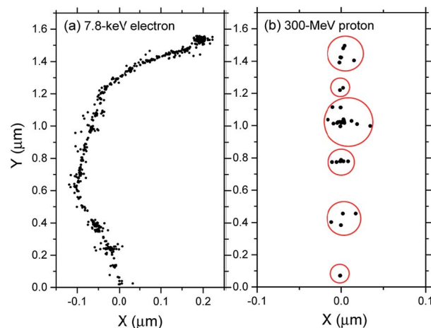
Fig. 1 Simulated track histories (projected into the XY plane of figure) of a 7.8 keV tritium \beta -electron (complete track; mean \text{LET} \sim 5.9 \text{ eV nm}^{-1} ) (panel a) and a 300 MeV proton (track segment; \text{LET} \sim 0.3 \text{ eV nm}^{-1} ) (panel b) incident in liquid water at 25 °C. The two irradiating particles are generated at the origin and start traveling along the Y axis. Dots represent the energy deposited at points where an interaction occurred.
