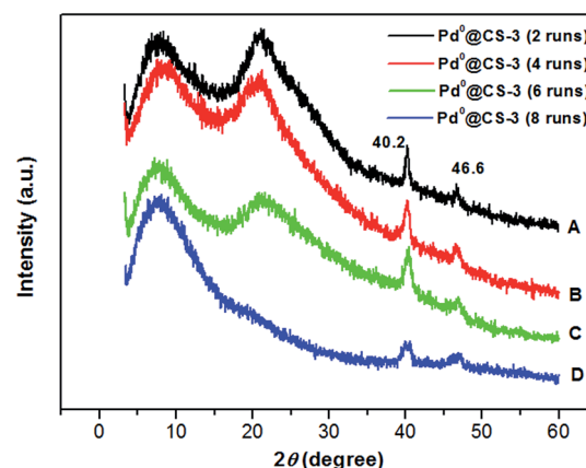
Fig. 6 XRD patterns of the reused \text{Pd}^0\text{@CS-3} membrane catalyst with different recycling runs.
