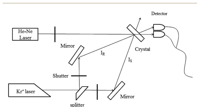
Fig. 3 Two-wavelength nonvolatile experiment setup.
