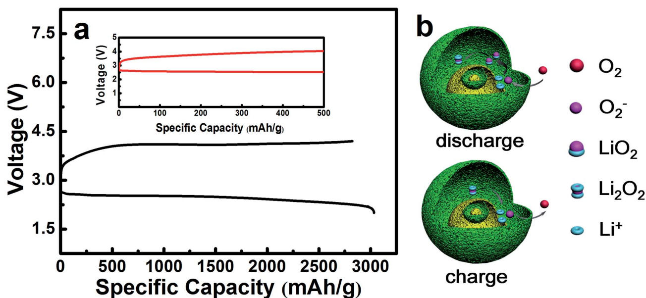
Fig. 6 (a) Galvanostatic discharge/charge curves of Li–O 2 batteries with a NiO catalyst at a current density of 0.1 \text{ mA cm}^{-2} in the voltage range of 2.0–4.2 V vs. \text{Li}^+/\text{Li} . (b) Illustration of the catalytic reaction mechanism for the layered nanosphere NiO in Li–O 2 batteries.
