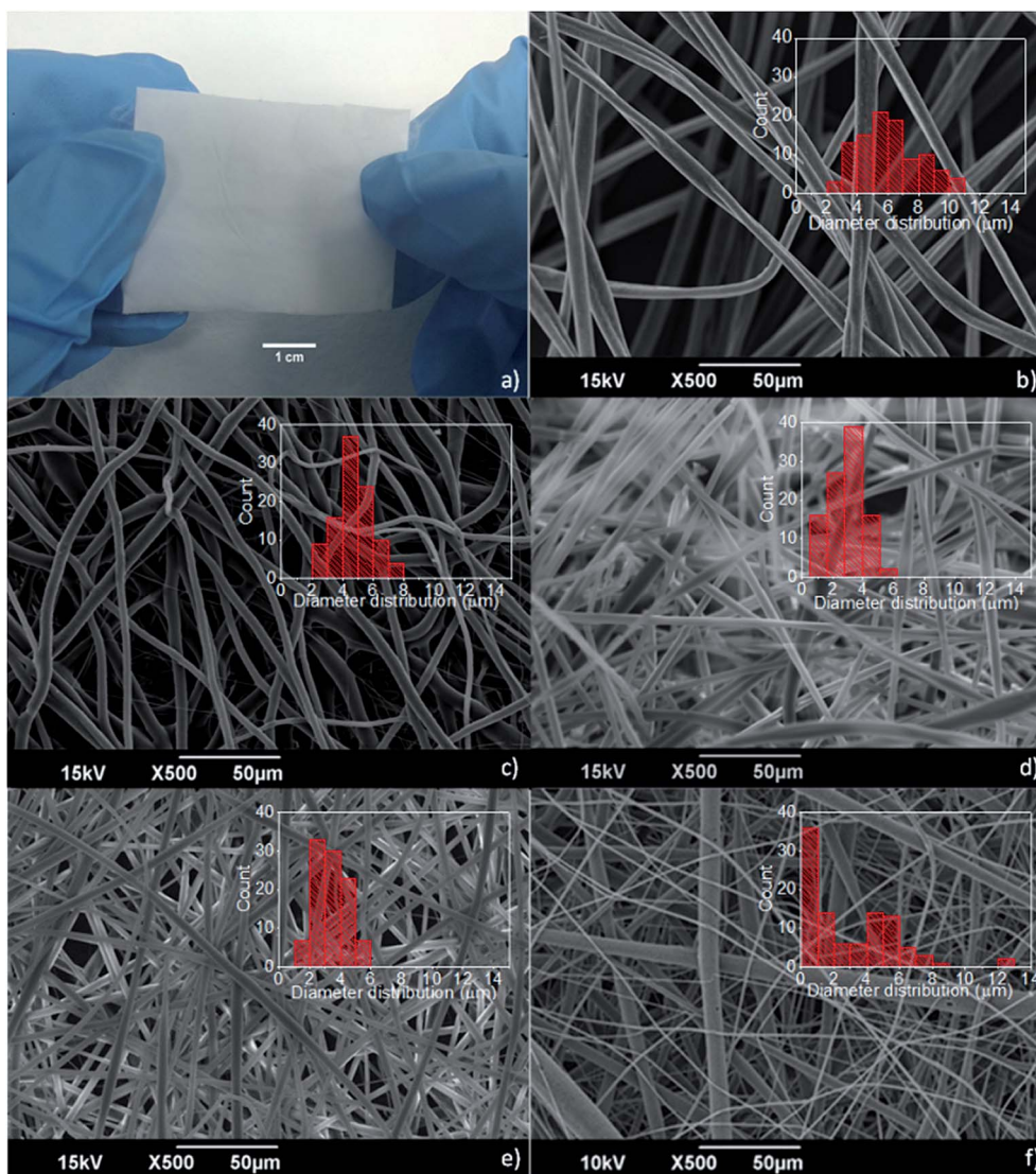
Fig. 1 (a) Photograph of the fibrous mat 50/50 PMMA/PCL, and SEM micrographs of fibrous mats: (b) PMMA, (c) PCL (d) 70/30 PMMA/PCL, (e) 50/50 PMMA/PCL, and (f) 30/70 PMMA/PCL. Insets: the diameter distributions of the fibers in each case.
