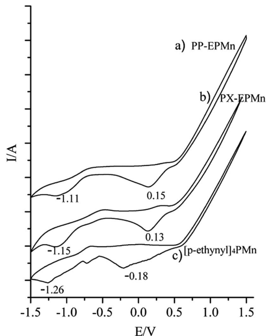
Fig. 5 Cyclic voltammetry curves of PP-EPMn (a), PX-EPMn (b) on the glass carbon electrodes in 0.1 \text{ mol L}^{-1} (\text{CH}_3\text{CH}_2)_4\text{NBr CH}_2\text{Cl}_2 solution; cyclic voltammetry curves of [p-ethynyl] _4 PMn (c) in \text{CH}_2\text{Cl}_2 , 0.1 \text{ mol L}^{-1} (\text{CH}_3\text{CH}_2)_4\text{NBr} . Scan rate 50 \text{ mV s}^{-1} .
