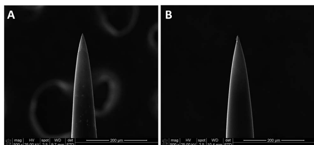
Fig. 3 Neural microelectrodes before (A) and after (B) vapor-deposition of polyionic nanocoating. Scale bar: 200 μm.
