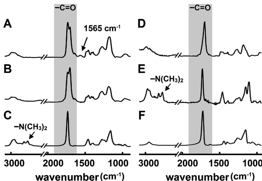
Fig. 2 FTIR spectra of hybrid polyionic nanocoatings of (A) PDME, (B) PME, and (C) PDE, compared with that of homopolymers of (D) PMAA, (E) PDMAEMA, and (F) PEGDA. The absorption peaks at 1702 cm -1 , 1728 cm -1 and 1735 cm -1 were assigned to C=O stretching of MAA, DMAEMA, and EGDA, respectively. The absorption peaks at 2772 and 2821 cm -1 were assigned to C-H stretching of tertiary amine in DMAEMA.
