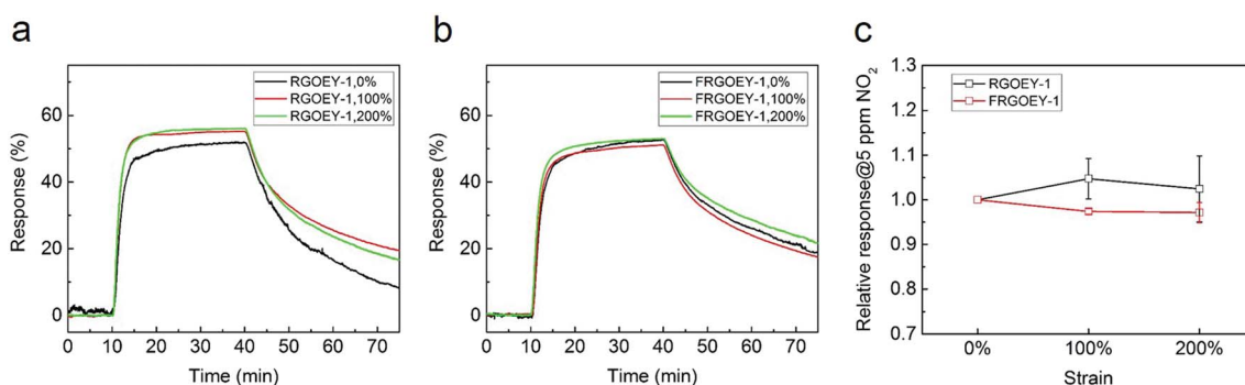
Fig. 4 (a and b) Gas sensing performances of RGOEY-1 and FRGOEY-1 exposed to 5.0 ppm NO 2 gas under 0%, 100%, and 200% strains. (c) Comparison of gas sensing performances of RGOEY-1 and FRGOEY-1 exposed to 5.0 ppm under 0%, 100%, and 200% strains.
