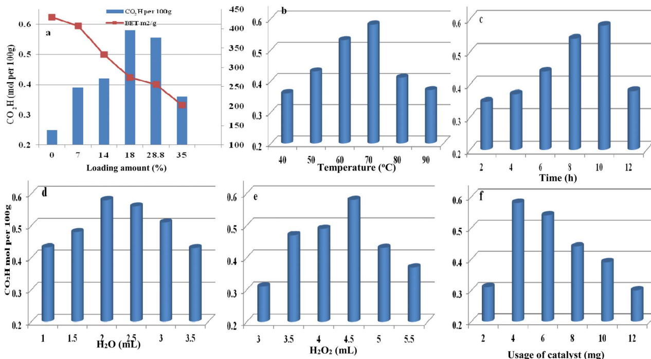
Fig. 8 Parameters affecting the oxidation reaction including different \text{H}_5\text{PMo}_{10}\text{V}_2\text{O}_{40} loading (a), temperature (b), time (c), water content (d), \text{H}_2\text{O}_2 dosage (e), and usage of catalyst (f).
