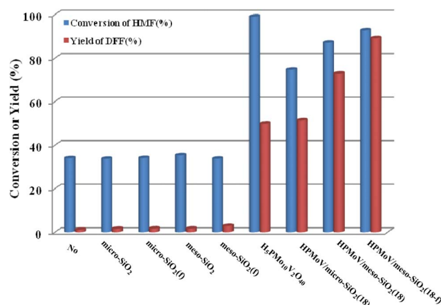
Fig. 9 Catalytic performance for various catalysts with different structures in oxidation of 5-HMF by \text{O}_2 . Reaction conditions: 1 mmol of 5-HMF, 80 mg of catalyst, and 5 mL solvent at 120^\circ\text{C} for 8 h.
