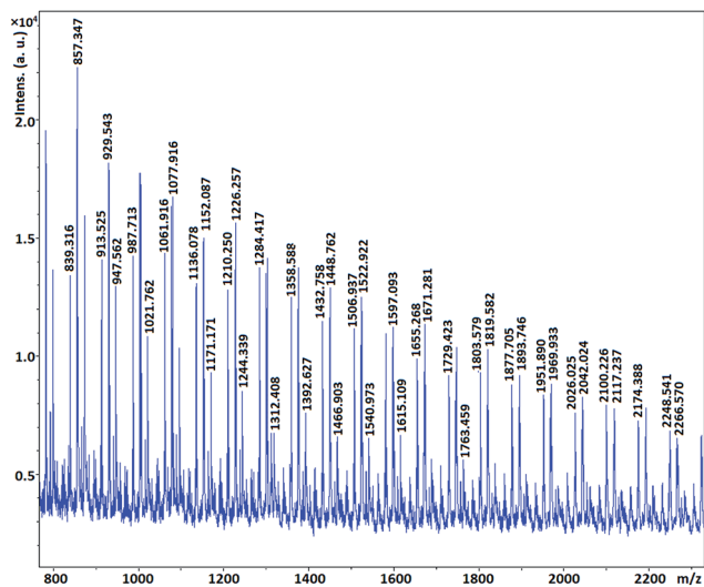
Fig. 7 MALDI-TOF mass spectra of hPG 3/70 .
