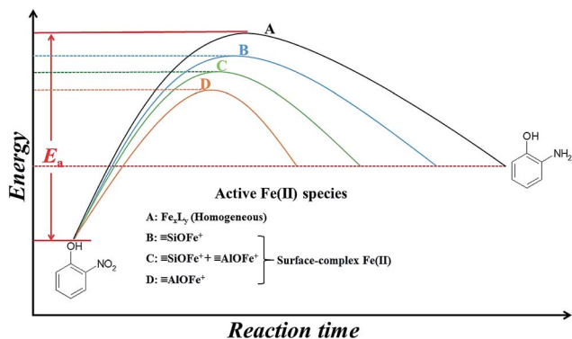
Fig. 6 The comparison of E_a and possible active [\equiv\text{Fe}(\text{III})]/[\equiv\text{Fe}(\text{II})] couples in 2-NP transformation under different reaction conditions.
