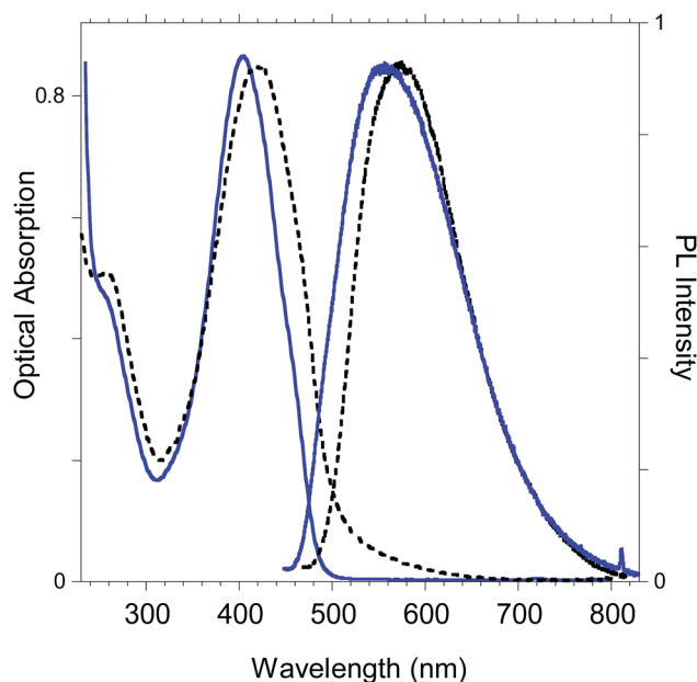
Fig. 11 Optical absorption and emission spectrum of poly-6-TT-BF3k in dichloromethane solutions (blue lines) and in the solid state (black lines).
