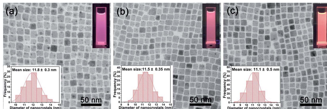
Fig. 8 Transmission electron microscope (TEM) images of the Mn-doped CsPb(Cl/Br) 3 NCs prepared at different reaction temperature: (a) 160 °C, (b) 180 °C, (c) 200 °C. Insets: corresponding particle size distribution and PL images excited by 365 nm UV light.
