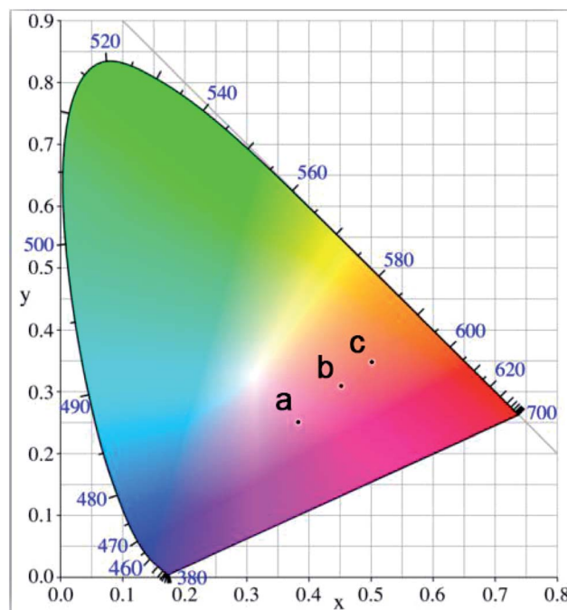
Fig. 9 CIE chromaticity diagram of the Mn-doped CsPb(Cl/Br) 3 NCs prepared at different reaction temperature: (a) 160 °C, (b) 180 °C, (c) 200 °C.
