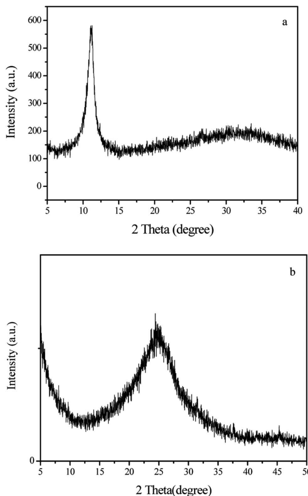
Fig. 3 XRD patterns of graphene oxide (a) and 3D-GA (b).
