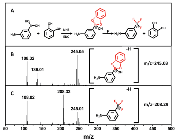
Fig. 2 (A) The mechanism of the boronate complex formation and F^- detection. (B) HR-MS spectrum of the boronate complex. (C) HR-MS spectrum of the boronate complex after the addition of F^- .
