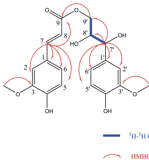
Fig. 3 Key ^1\text{H}-^1\text{H} COSY and HMBC correlations of compound 4.
