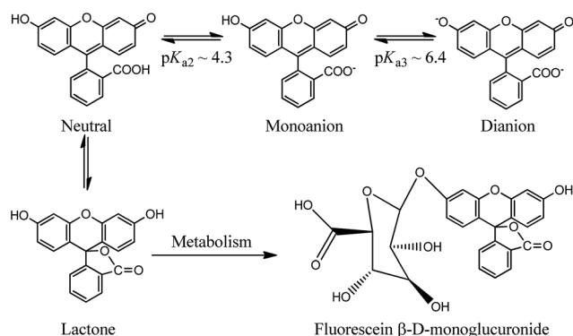
Scheme 1 Prototypes of FL and the metabolism to fluorescein \beta -D-monoglucuronide.
