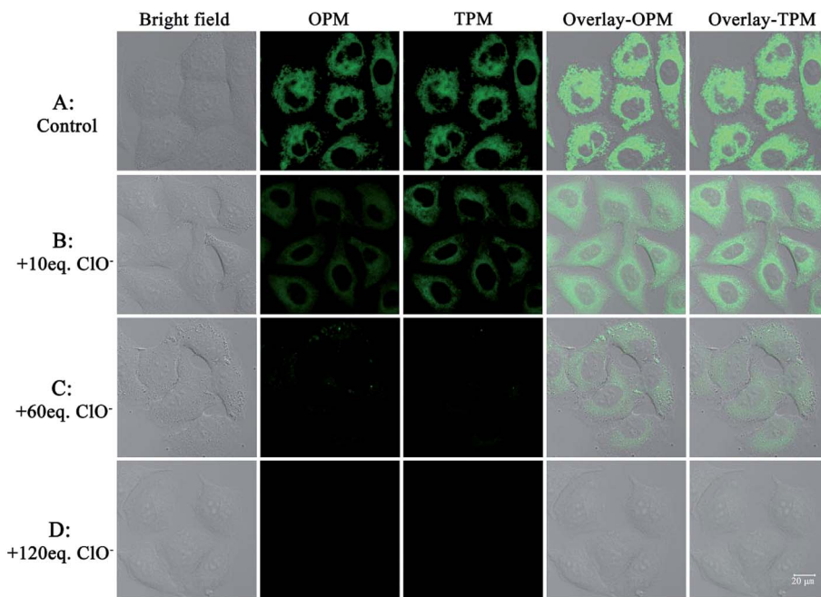
Fig. 5 One-photon and two-photon microscopy (OPM, TPM) confocal fluorescence images of A549 cells. Images of cells incubated with probe 1 (20 \mu M) for 30 min (control. (A)). Images of cells incubated with probe 1 for 30 min and subsequently with \text{ClO}^- (10 equiv., (B); 60 equiv., (C); 120 equiv., (D)). The probe was excited at 458 nm (OPM) or 810 nm (TPM). The emission was collected at 520 \pm 30 nm. Overlay-OPM: overlay of bright field and OPM columns. Overlay-TPM: overlay of bright field and TPM columns.
