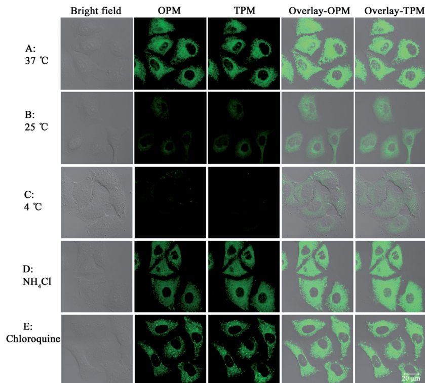
Fig. 4 Confocal images of A549 cells incubated with 1 (20 \mu M) under different conditions. (A)–(C): cells were incubated with 1 at 37 ^{\circ} C (A), 25 ^{\circ} C (B) or 4 ^{\circ} C (C) for 30 min. (D) and (E): cells were preincubated with \text{NH}_4\text{Cl} (50 \mu M) or chloroquine (10 \mu M) for 1 h at 37 ^{\circ} C and then incubated with 1 (20 \mu M) for 30 min, respectively. The probe was excited at 458 nm (OPM) or 810 nm (TPM). The emission was collected at 520 \pm 30 nm. Overlay-OPM: overlay of the bright field and OPM columns. Overlay-TPM: overlay of the bright field and TPM columns.
