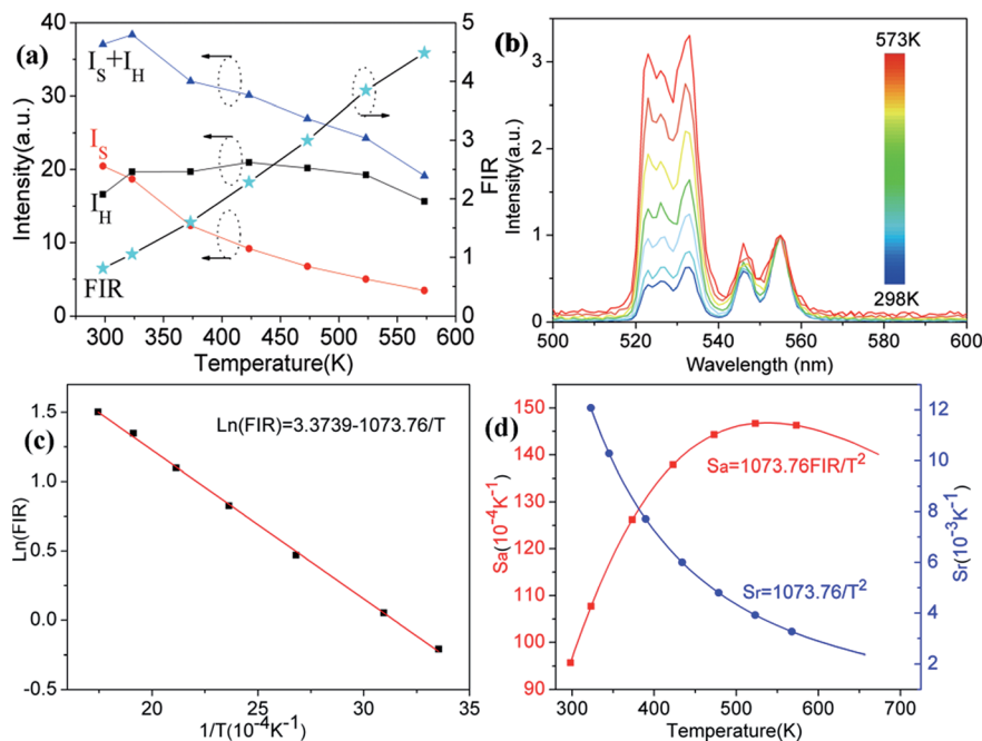
Fig. 6 (a) Integrated upconversion intensities of ^2\text{H}_{11/2} ( I_H ) and ^4\text{S}_{3/2} ( I_S ) as well as FIR versus temperature; (b) normalized upconversion luminescence of \text{Er}^{3+} at a temperature range of 298–573 K; (c) \ln(\text{FIR}) as a function of the inverse absolute temperature 1/T ; (d) temperature sensitivity versus absolute temperature.
