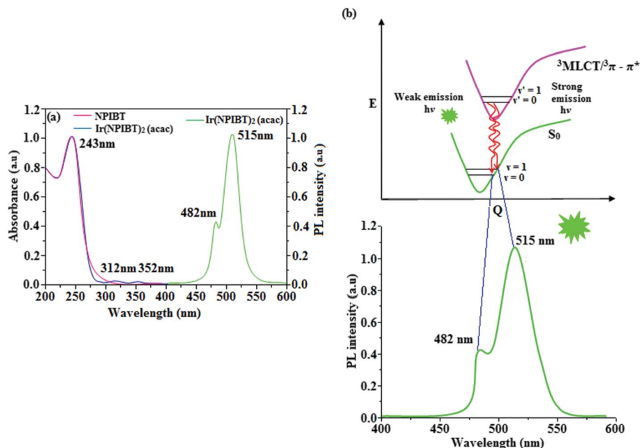
Fig. 5 (a) UV and PL spectra of NPIBT and \text{Ir}(\text{NPIBT})_2(\text{acac}) ; (b) representative Franck–Condon electronic transitions of \text{Ir}(\text{NPIBT})_2(\text{acac}) .
