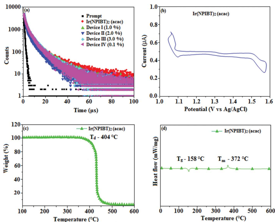
Fig. 6 (a) Life time spectra of \text{Ir}(\text{NPIBT})_2(\text{acac}) , device I–IV; (b) cyclic voltammogram of \text{Ir}(\text{NPIBT})_2(\text{acac}) ; (c) TGA and (d) DSC of \text{Ir}(\text{NPIBT})_2(\text{acac}) .
