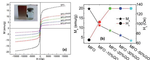
Fig. 6 (a) Room temperature magnetic hysteresis (M-H) curves for bare MnFe 2 O 4 nanoparticles and GO-MnFe 2 O 4 nanocomposites and (b) the saturation magnetization (M s ) and coercivity (H c ) values determined from the magnetic hysteresis curves. The inset of (a) demonstrates the magnetic separation ability of MFO-GO sample by using a small magnet.
