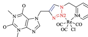
C22H22ClN8O6Re
