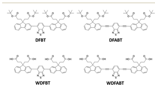
Scheme 1 Chemical structure of DFBT , DFABT , WDFBT and WDFABT .
