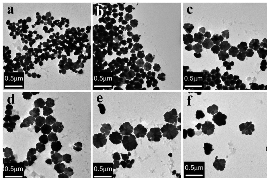
Fig. 10 TEM images of silver nanoparticle products synthesized from the extract of Flos Magnoliae officinalis : (a) 2.5 \text{ g L}^{-1} ; (b) 5 \text{ g L}^{-1} ; (c) 10 \text{ g L}^{-1} ; (d) 20 \text{ g L}^{-1} ; (e) 30 \text{ g L}^{-1} ; (f) 40 \text{ g L}^{-1} . 81
