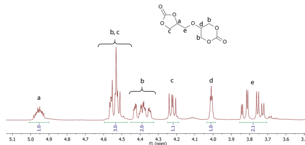
Fig. 1 ^1\text{H} NMR of 56BCC.
