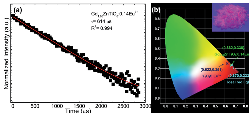
Fig. 8 (a) Luminescence decay curve and (b) CIE chromaticity coordinate of the Gd_{1.86}ZnTiO_6:0.14Eu^{3+} phosphor. The vivid and intense red color was clearly observed from the powders by naked-eyes as shown in the photograph of (b).
