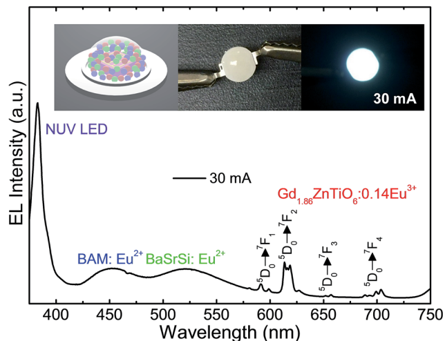
Fig. 9 EL spectrum of the WLED fabricated by the combination of UV LED ( \lambda \sim 385 nm), commercial blue-emitting and green-emitting phosphors, and Gd_{1.86}ZnTiO_6:0.14Eu^{3+} red-emitting phosphor at the injection current of 30 mA under continuous-wave mode. The schematic illustration of WLED and its photographs before/after the current injection were demonstrated in the inset.
