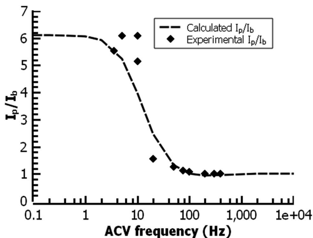
Fig. 11 ACV analysis of a ferrocene-functionalized film deposited from ACN (30 min.) on ITO. The fit gives a rate constant for the redox reaction of 30 \text{ s}^{-1} .
