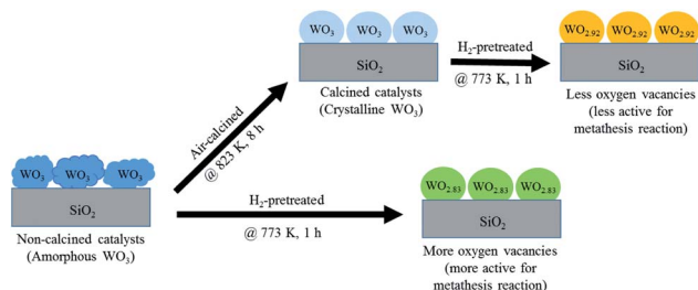
Scheme 2 The summarized results of the non-calcined and air-calcined catalysts with H 2 pretreatment.
