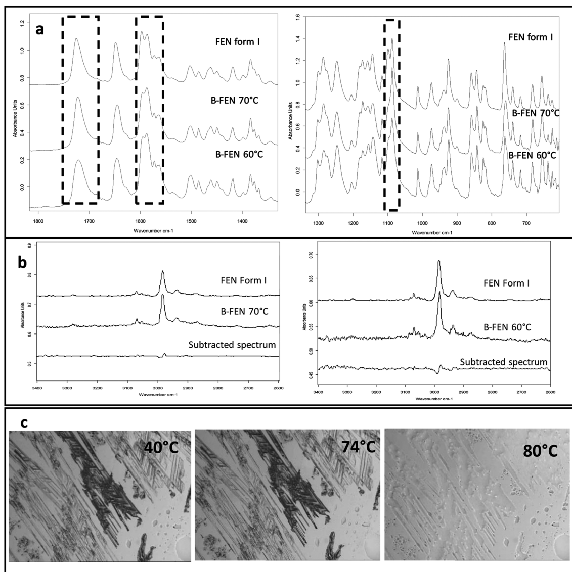
Fig. 8 ATR-FTIR spectra of (a) B-FEN 60 and 70 °C in comparison to the reference form I spectrum (1800–600 cm⁻¹); (b) the subtracted spectra of B-FEN 60 and 70 °C from the form I spectrum at 3400 to 2600 cm⁻¹; (c) HS-PLM images of B-FEN 70 °C heated to 40, 74 and 80 °C.
