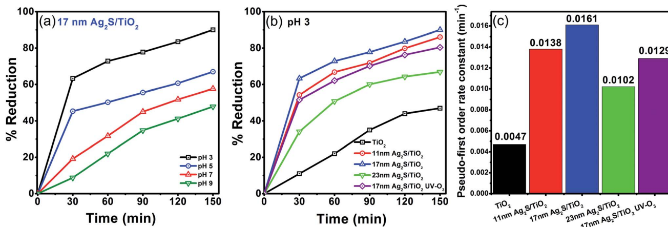
Fig. 3 (a) Photo-reduction of Cr(vi) at different pH values using 17 nm \text{Ag}_2\text{S}/\text{TiO}_2 nanofibers, (b) photo-reduction using variable sized \text{Ag}_2\text{S}/\text{TiO}_2 nanofibers at pH 3 compared to the pristine \text{TiO}_2 nanofibers, and (c) the corresponding pseudo-first order rate constants.
