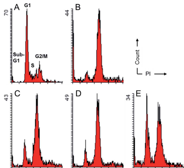
Fig. 3 Effects of compounds 2a, 2d and 3b on cell cycle progression. MDA-MB-231 cells were treated for 24 h with compounds at a concentration five-fold GI_{50} . Cells were fixed and stained with propidium iodide (PI) followed by cell cycle analysis using a flow cytometer. DMSO (A) and 200 nM combretastatin A-4 (CA-4) (B) were used as negative and positive control, respectively, for induction of cell cycle arrest in G2/M. Compounds 2a at 6.0 \mu M (C), 2d at 8.0 \mu M (D) or 3b at 10.5 \mu M (E) were used.
