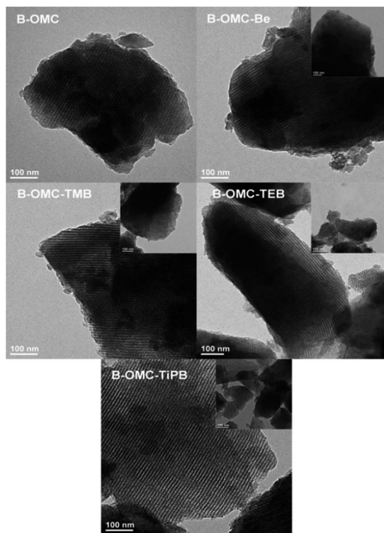
Fig. 2 TEM images of the B-OMCs with different expanding agents, calcined at 800 °C under N 2 .
