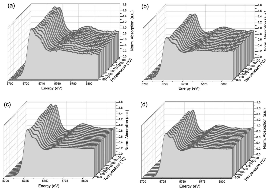
Fig. 3 In situ XANES profiles collected upon heating in 5 mol% \text{H}_2/\text{He} for samples: (a) CuO–NiO/ZDC, (b) NiO/ZDC, (c) CuO/ZDC, and (d) ZDC.
