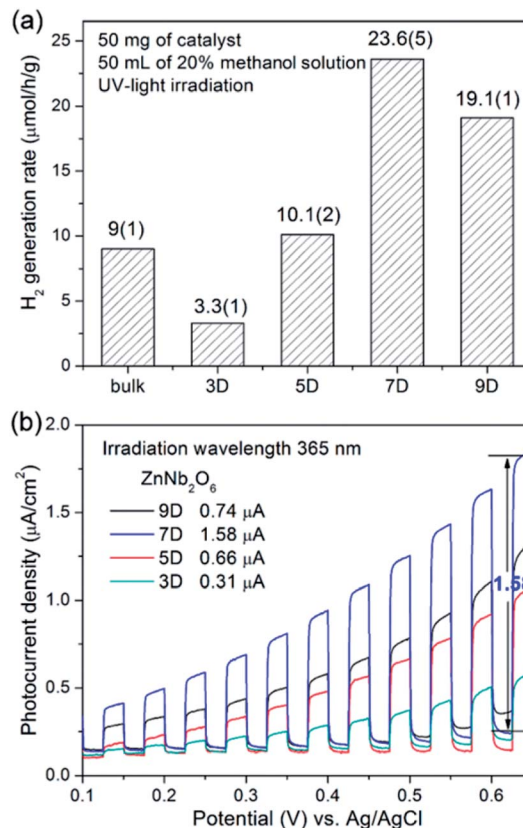
Fig. 6 (a) Photocatalytic H 2 generation rates of bulk-ZnNb 2 O 6 and nano-ZnNb 2 O 6 synthesized hydrothermally for 3, 5, 7, and 9 days, (b) photoelectrochemical responses using a three-electrode setup in 0.1 M Na 2 SO 4 aqueous solution.
