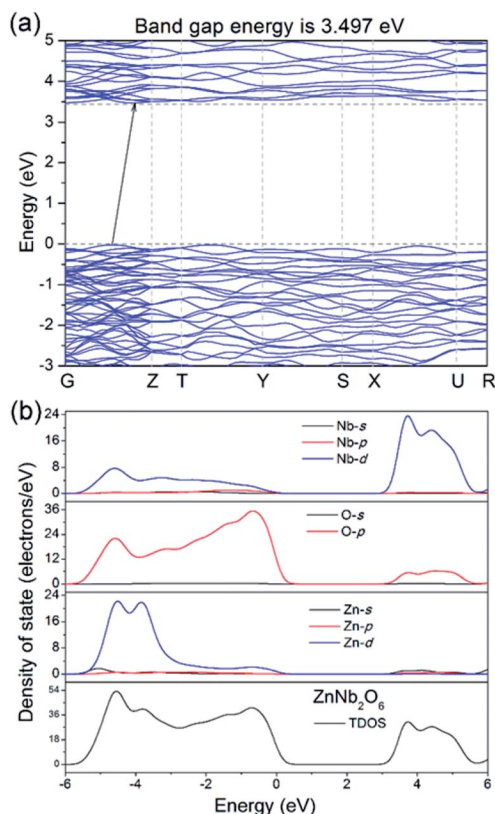
Fig. 4 (a) Calculated energy band structure of ZnNb 2 O 6 , (b) partial and total density of state in the range from -6 to 6 eV.
