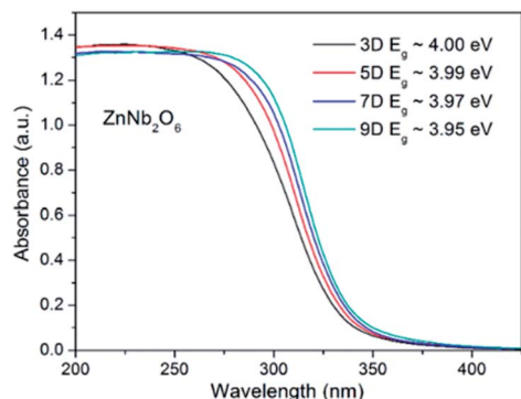
Fig. 3 UV-Vis reflectance spectra of ZnNb 2 O 6 -3D, -5D, -7D, and -9D. The bandgap energies provided here were estimated from their differential curves.
