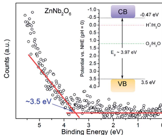
Fig. 5 Potential of valence electron for ZnNb 2 O 6 was estimated according to the rising point in ultraviolet photoelectron spectrum, and the proposed band structure potentials are provided as the inset.
